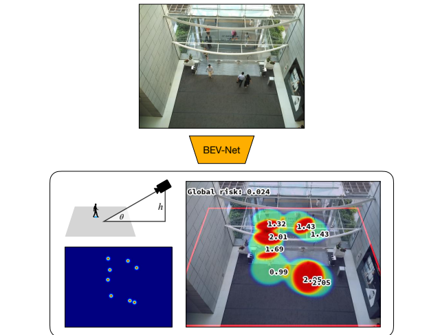
Figure 1: Set of tasks proposed for social distancing compliance assessment. Given an input image, models are expected to jointly predict camera geometry (top left), bird's eye view heatmap of person locations (bottom left), local risk map highlighting areas with high probability of infection (right), as well as individual and global risk level for the entire scene (annotated over the risk map).
